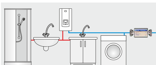
Magnetyzer Megamax 3/4"
